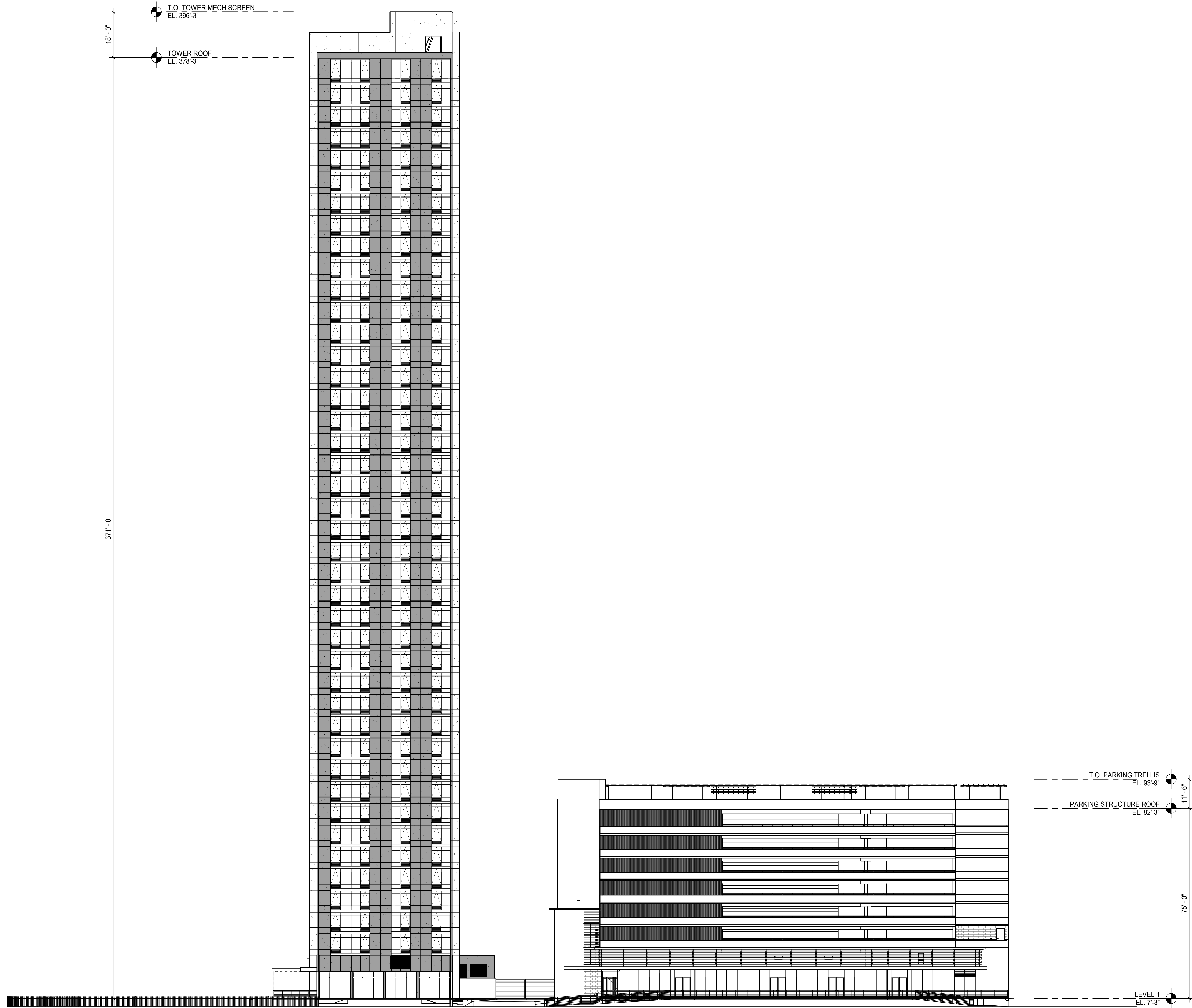
1 NORTH ELEVATION (MAUKA) SCALE: 1/16" = 1'-0" 1/16" = 1'-0"
