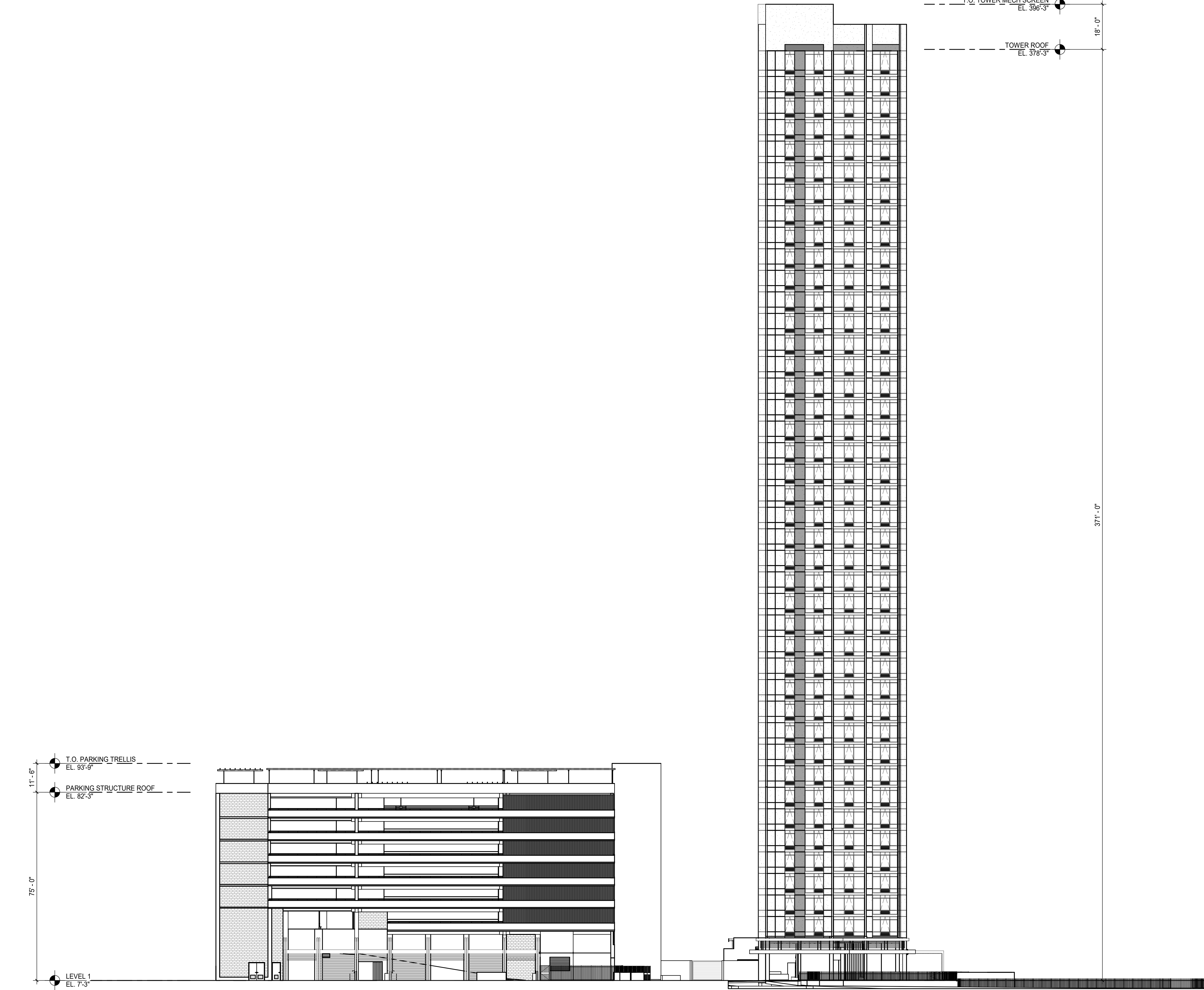
1 SOUTH ELEVATION (MAKAI) SCALE: 1/16" = 1'-0"
